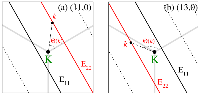
Figure 4.4 Cutting lines for (a) (11,0) and (b) (13,0) zigzag nanotubes near the graphene K-point. Solid lines denote the E_{11} and E_{22} cutting lines, while the dotted lines correspond to higher cutting lines. The angle \Theta(\mathbf{k}) is measured counterclockwise from a line perpendicular to the cutting lines, where the positive direction of the line is to the right of the K-point. Here \Theta(\mathbf{k}) is shown for a k point on the E_{22} cutting line for both SWNTs. The difference between the type-I and type-II families can be understood from the position of the E_{11} or E_{22} cutting lines relative to the K-point [73].
