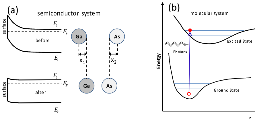
Figure 1.3 Generation mechanisms for coherent phonons. (a) A conventional polar semiconductor like GaAs. Before photoexcitation by the pump pulse, the surface depletion field cause the Ga and As ions to be displaced by an amount x_1 and x_2 from their equilibrium (no depletion field) position. After photoexcitation, the electrons and holes generated near the surface will screen the depletion field, causing the Ga and As ions to return to their equilibrium position, and trigger the coherent phonon. (b) A typical molecule. The combined electronic and vibrational energy levels for the grounds state energy surface and an excited state energy surface are shown. The ground state and excited state energy surfaces have different minima, and thus photoexcitation by the pump pulse from the grounds state to the excited state triggers the coherent phonon and the system wants to move to a new minima.
