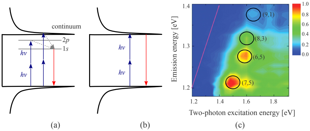
Figure 1.9 Two-photon experiment by Wang et al. [27]. (a) In the exciton picture, the 1s exciton state is forbidden under two-photon excitation. The 2p exciton and continuum states are excited. They relax to the 1s exciton state and fluoresce through a one-photon process. (b) In the simple band picture, two-photon excitation energy is the same as emission energy, but this case is not observed. (c) Contour plot of two-photon excitation spectra of SWNTs. By comparison with the solid line describing equal excitation and emission energies, it is clear that the two-photon excitation peaks are shifted above the energy of the corresponding emission feature. The large shift arises from the excitonic nature of the nanotube optical transitions. E_{bd} is found to be as large as up to 1 eV, thus excitons play an important role in the nanotube optics.
