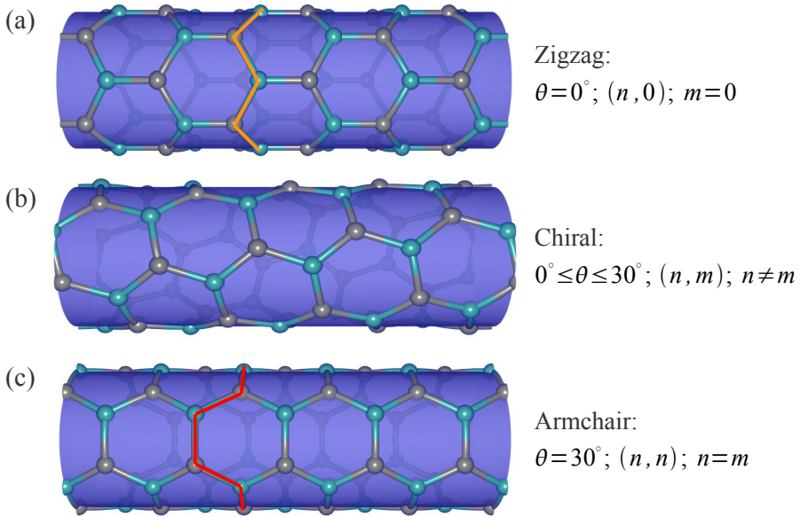
Figure 2.3 Classification of carbon nanotubes: (a) zigzag, (b) chiral, (c) armchair SWNTs. From left to right, the chiral index of each SWNT above is (5,0) , (4,2) , (3,3) , respectively. In (a) and (c), thick solid lines are to emphasize “zigzag” and “armchair” structures, respectively.
