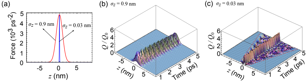
Figure 5.5 (a) Driving forces with two different parameters \sigma_z (= 0.9 \text{ nm}) > \sigma_{zc} and \sigma_z (= 0.03 \text{ nm}) < \sigma_{zc} , which give (b) only localized and (c) localized and propagating wave components, respectively. For the (11,0) tube in this simulation, we have \sigma_{zc} = 0.045 \text{ nm} . The propagating wave components in (c) travel with a speed of 1.68 \text{ nm/ps} , as indicated by the slope of the dashed line.
