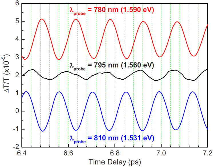
Figure 1.6 Differential transmission as a function of time delay at probe wavelengths of 780, 795, and 810 nm for the selective RBM excitation of the (11, 3) nanotube. There is a \pi -phase shift between the 780 and 810 nm data. These three wavelengths (from the top to the bottom of the figure) correspond to photon energies above, at, and below the energy of the second exciton resonance, respectively, of the (11, 3) nanotube. Reproduced from Ref. [8].
