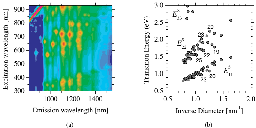
Figure 2.13 (a) 2D photoluminescence (PL) map measured on wrapped HiPco SWNTs suspended by SDS surfactant in aqueous solution [40]. (b) The Kataura plot extracted from the PL map [25]. The numbers show the constant 2n+m families. Reproduced from Ref. [38].
