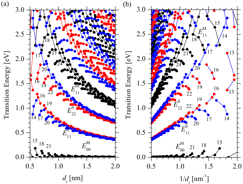
Figure 2.15 The ETB Kataura plot similar to the STB Kataura plot in Fig. 2.12 as a function of (a) SWNT diameter d_t , and (b) inverse diameter 1/d_t . The ETB model takes into account the long-range atomic interactions, the curvature effects of small diameter SWNTs, and the optimized geometrical structures of the SWNTs. Black, red, and blue dots correspond to M-, S1-, and S2 SWNTs, respectively. The constant 2n + m families are connected by lines. Reproduced from Ref. [38].
