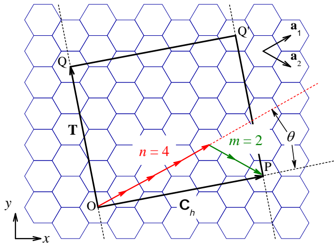
Figure 2.2 Geometry of a (4,2) SWNT viewed as an unrolled graphene sheet with the graphene unit vectors \mathbf{a}_1 and \mathbf{a}_2 . The rectangle OPQ'Q is the 1D SWNT unit cell. Total hexagons covered within this rectangle unit cell is N = 28 . \mathbf{OP} and \mathbf{OQ} define the chiral vector \mathbf{C}_h and translation vector \mathbf{T} , respectively, whereas the chiral angle \theta is the angle between \mathbf{a}_1 and \mathbf{C}_h . From the figure, it is obvious \mathbf{C}_h = (4, 2) and \mathbf{T} = (4, -5) . If the site O is connected to P , and the site Q is connected to Q' , the cylindrical SWNT can be constructed.
