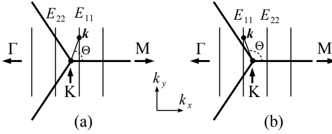
Figure 4.7 Cutting lines for (a) mod 0 aGNR and (b) mod 1 aGNRs near the Dirac K point. To make clear the definition of \Theta(k) , in this figure \Theta(k) is shown for an arbitrary \mathbf{k} at E_{11} . In fact, in the case of mod 0 and mod 1 aGNRs the E_{11} transitions occur at \Theta(k) = 0 and \Theta(k) = \pi , respectively. The difference between the mod 0 and mod 1 aGNRs can be understood from the position of the E_{11} or E_{22} cutting lines relative to the K point.
