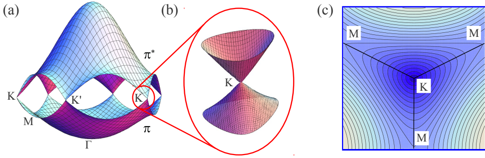
Figure 2.6 The \pi bands of graphene within the simple tight-binding method. In (a), the energy dispersion is shown throughout the whole region of the Brillouin zone. (b) Near the K point, the energy dispersion relation is approximately linear, showing two symmetric cone shapes, the so-called Dirac cones. (c) Contour plot of the energy dispersion near the K point. The tight-binding parameters used here are \varepsilon_{2p} = 0 eV, t = -3.033 eV, and s = 0.129 .
