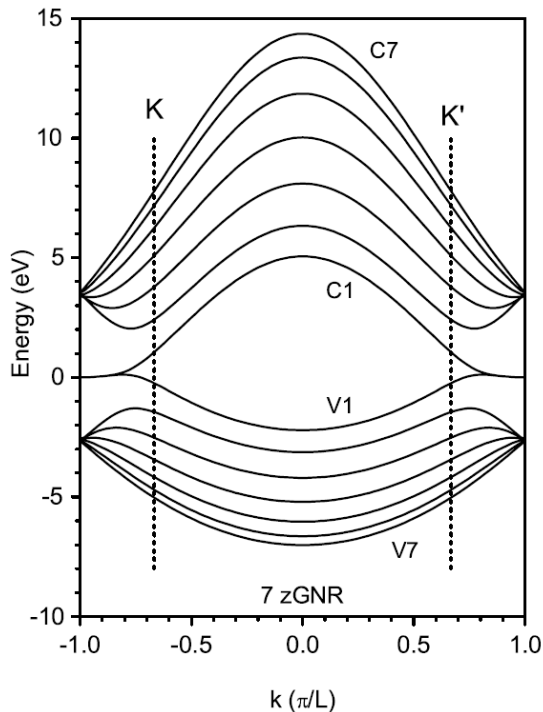
Figure 2.17 Electronic energy bands a 7-zGNR nanoribbon calculated in the ETB model. The lowest seven bands labeled v1 \dots v7 are the valence bands, while the highest seven bands labeled c1 \dots c7 are the conduction bands.
