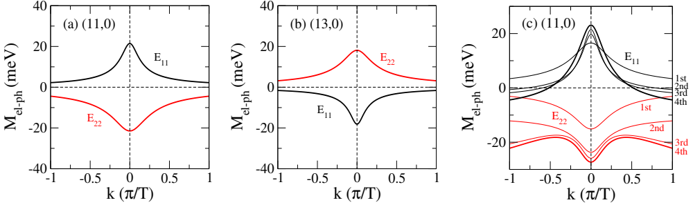
Figure 4.5 RBM electron-phonon matrix elements of (a) (11, 0) and (b) (13, 0) nanotubes calculated within the effective-mass theory using g_{\text{off}} = 6.4 \text{ eV} . In panels (a) and (b), the matrix elements near k = 0 are comparable with the results in Fig. 4.2. Panel (c) shows the matrix elements of an (11, 0) nanotube calculated within the ETB model for interactions up to the fourth nearest-neighbors. The results including fourth nearest neighbors exactly reproduce the results in Fig. 4.2(a).
