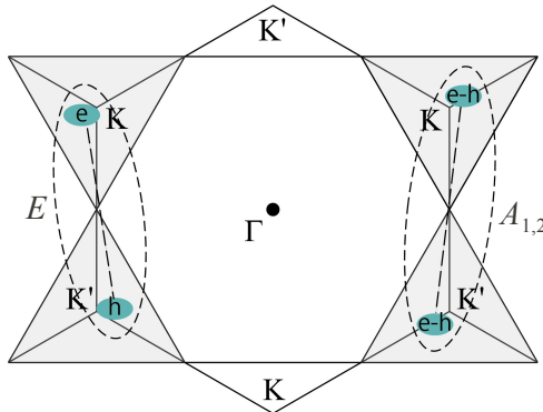
Figure 2.22 Symmetry of an exciton. If both the electron and hole are from the K (or K') region (right side of the above figure), the corresponding exciton is an A_{1,2} symmetry exciton. If an electron is from the K region and a hole is from the K' region (left side of the above figure), the corresponding exciton is an E symmetry. One more case is not shown here, the E^* exciton, which is just an opposite situation of the E exciton.
