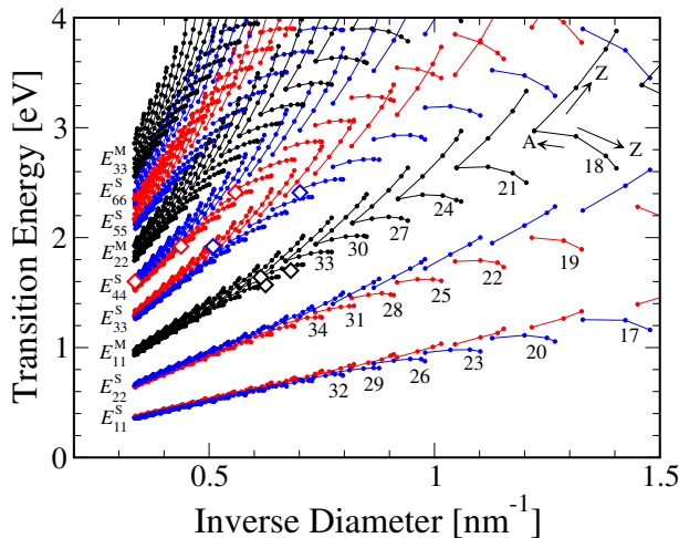
Figure 2.24 The bright exciton energy Kataura plot as a function of inverse diameter 1/d_t for \kappa = 2.22 . The exciton energies E_{ii} shown here are up to E_{66}^S and E_{33}^M . Black, red, and blue dots correspond to M-, S1-, and S2 SWNTs, respectively. The eight diamond symbols are experimental data by Michel et al. (Ref. [61]). The 2n + m family patterns are clearly seen for smaller diameter SWNTs. The arrows with A (Z) symbols correspond to the near armchair (zigzag) SWNTs.
