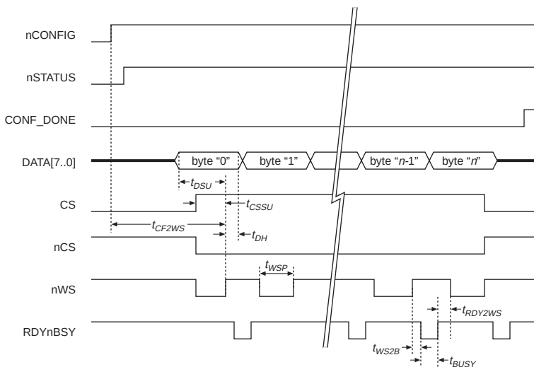
Figure 12. Passive Parallel Asynchronous Timing Waveforms
