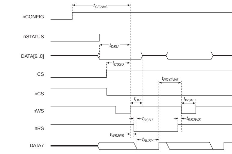
Figure 13. Passive Parallel Asynchronous Timing Waveforms Using nRS & DATA7
