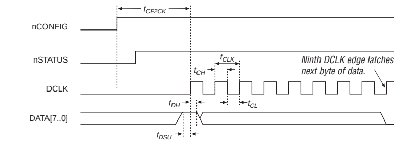
Figure 10. Passive Parallel Synchronous Configuration Timing Waveforms
