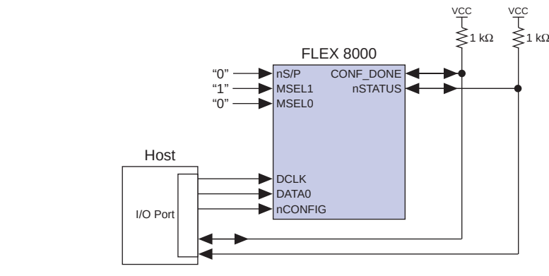
Figure 17. Bit-Wide Passive Serial Device Configuration
