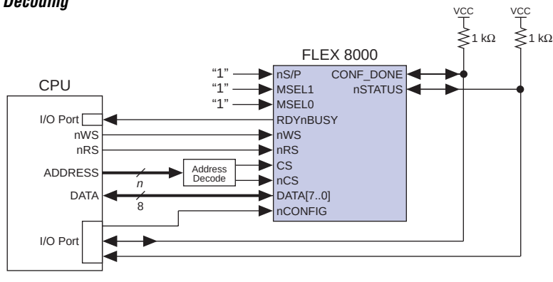
Figure 14. Passive Parallel Asynchronous Device Configuration with Address Decoding
