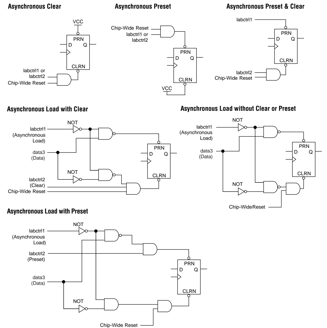
Figure 12. FLEX 10KE LE Clear & Preset Modes
