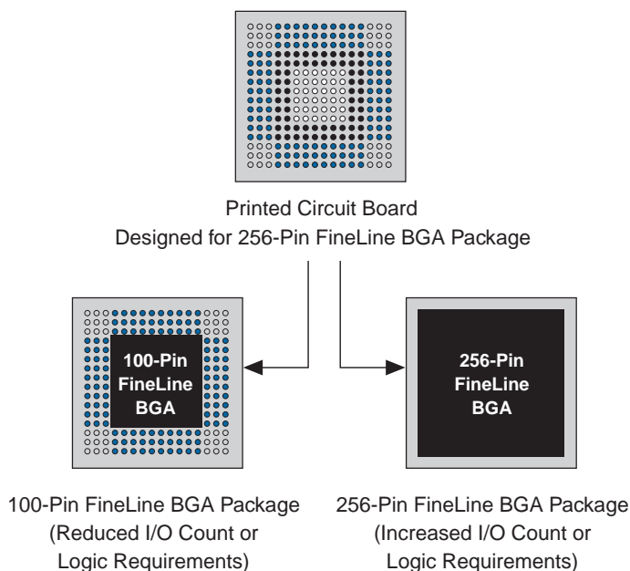
Figure 18. SameFrame Pin-Out Example
