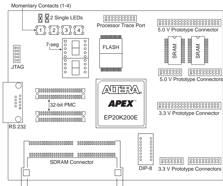
Figure 3. Excalibur Development Board
