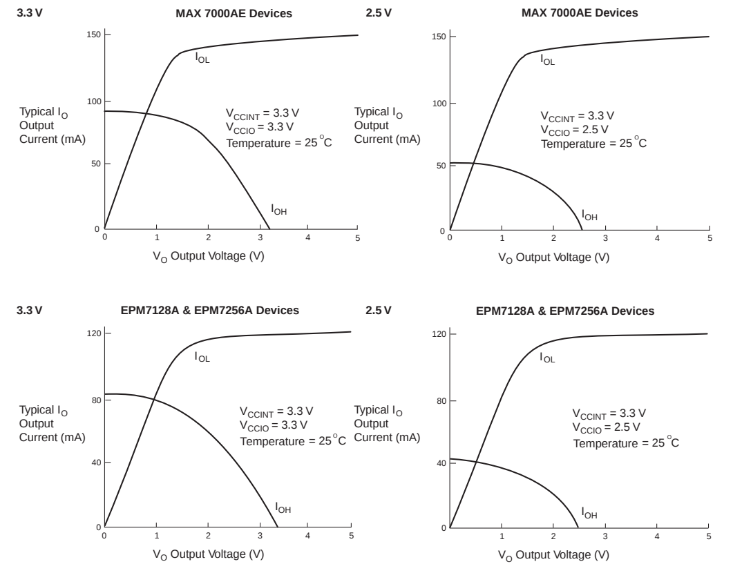
Figure 10. Output Drive Characteristics of MAX 7000A Devices
