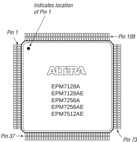
Figure 18. 144-Pin TQFP Package Pin-Out Diagram
