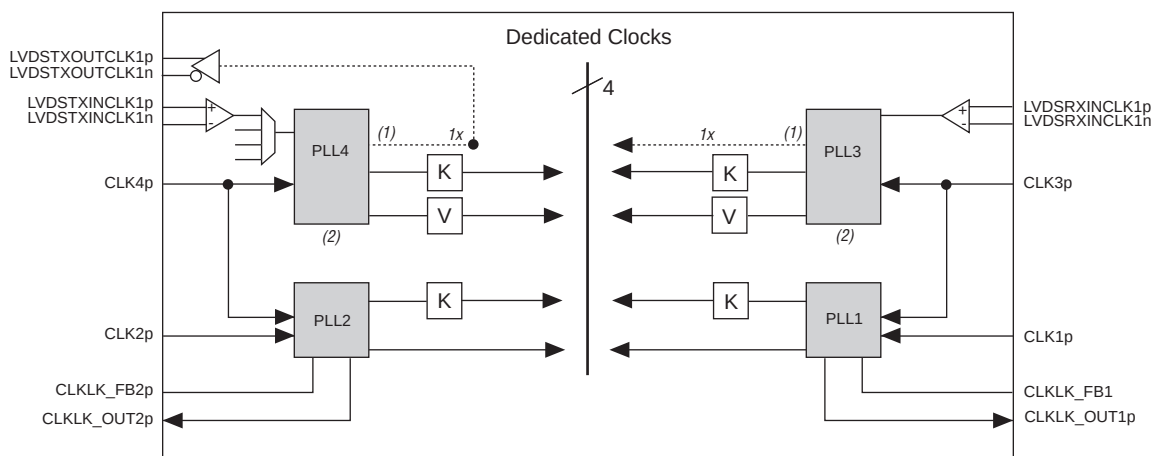
Figure 2. LVDS PLL Block Diagram
