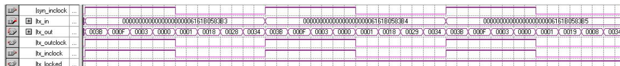
Figure 22. Example Functional Simulation Waveform of LVDS Transmitter
