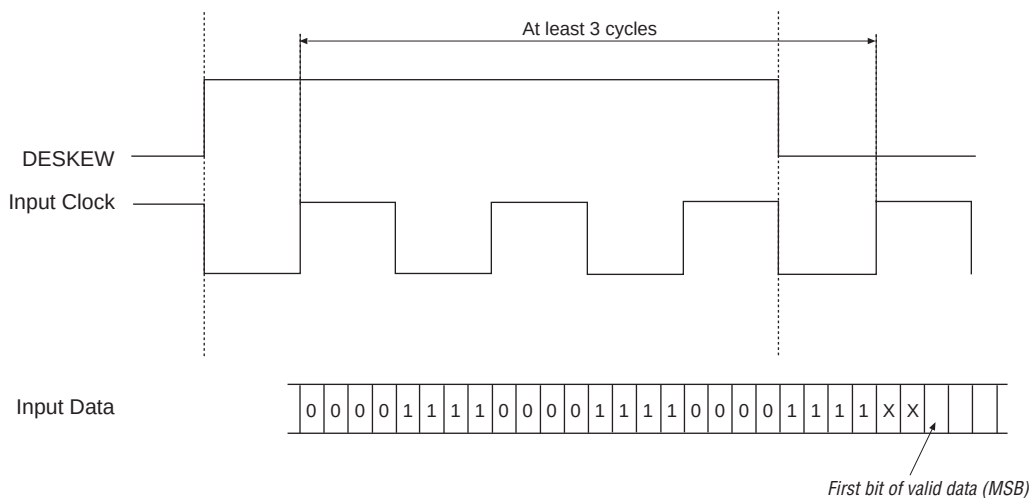
Figure 4. Deskew Circuitry Calibration Waveform for 8× Mode
