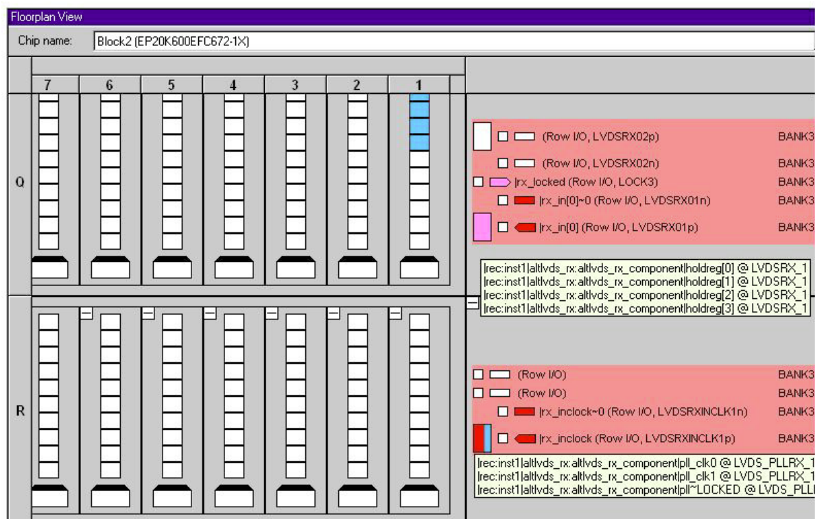
Figure 21. Floorplanner View of LVDS Receiver
