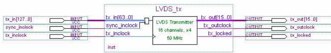
Figure 12. 50 MHz 16-Channel 4x LVDS Transmitter
